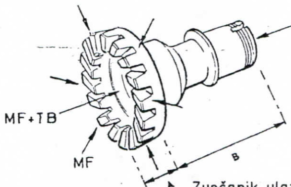
Zupčanik ulaza snage (17)
