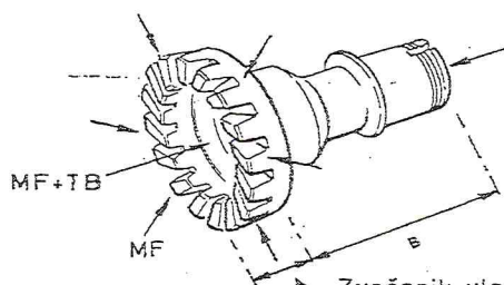
Zupčanik ulaza snage (17)
