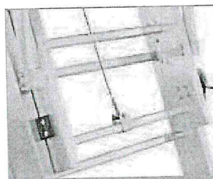
Height adjustment in rung grid of 280 mm
